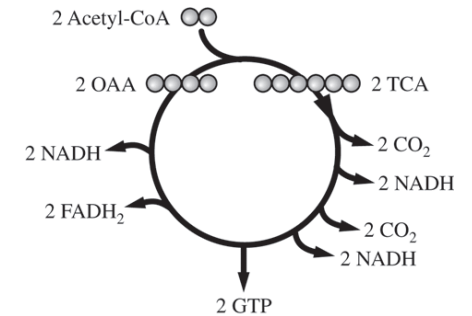
Figure 2. Krebs cycle
