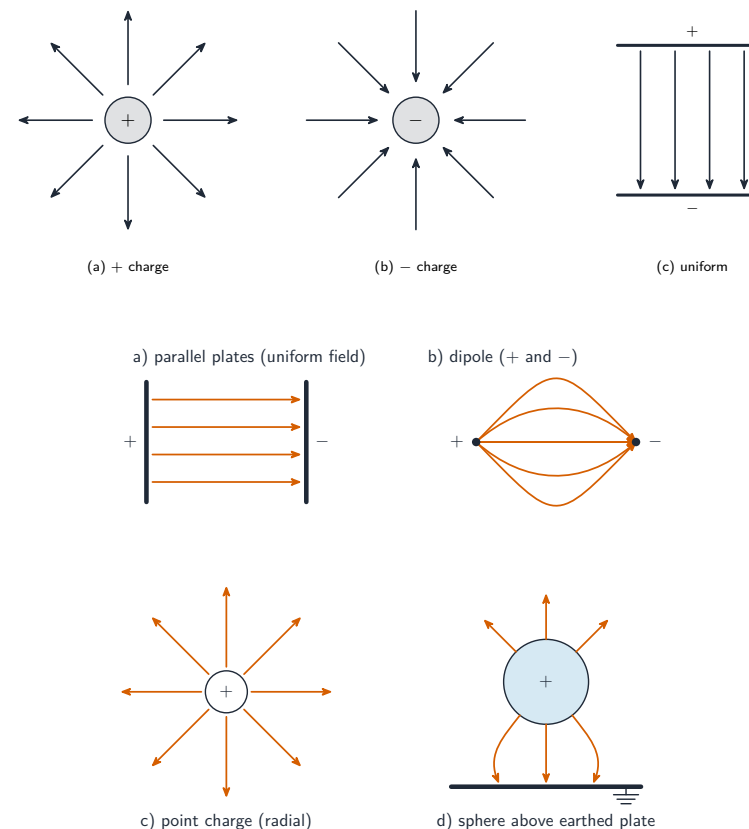
Electric field line patterns
