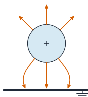
d) sphere above earthed plate
