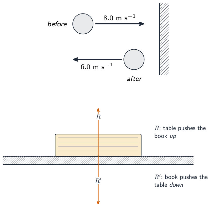
Newton third-law force pairs
