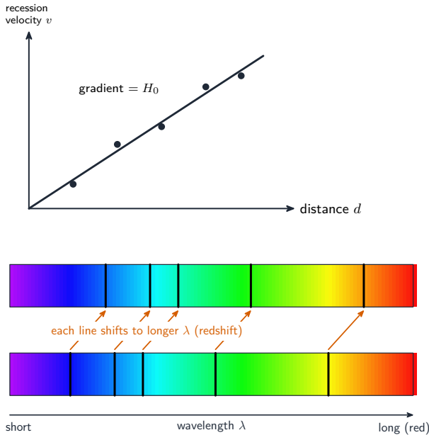
Redshift in a galaxy spectrum
