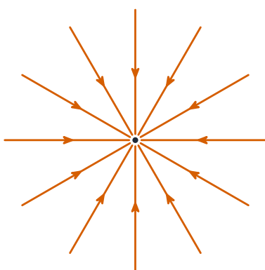
point mass
