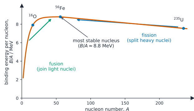
binding energy per nucleon peaks near ^{56}\text{Fe}
