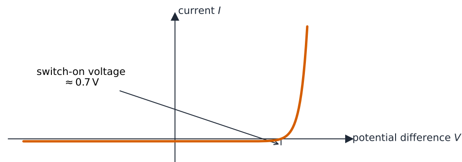
Si diode: conducts above \approx 0.7 V · reverse blocks
