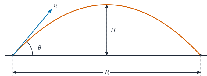
Range R of a projectile launched from and landing on level ground
