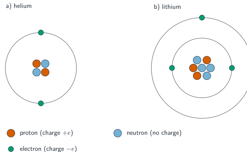
Simple models of a helium atom and a lithium atom (not to scale)
