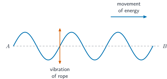
Transverse wave on a rope
