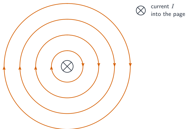
circular field lines (right-hand grip rule)
