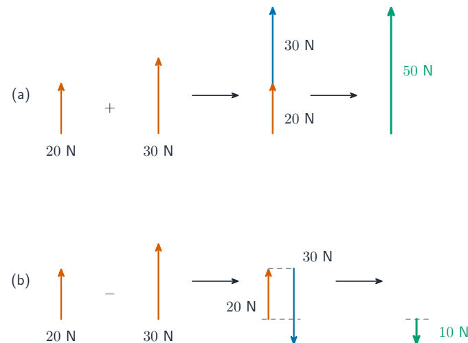
Adding and subtracting parallel vectors
