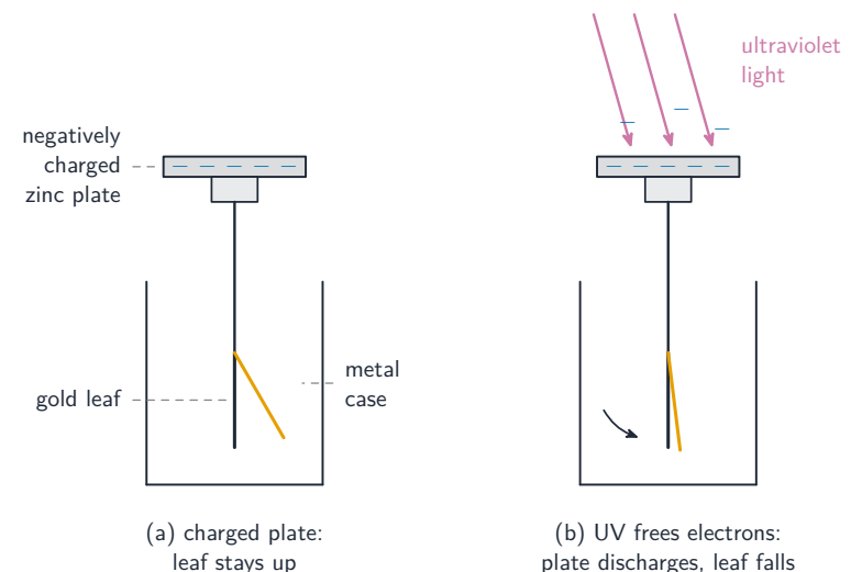
A charged zinc plate loses its charge — the gold leaf falls — when ultraviolet light shines on it
