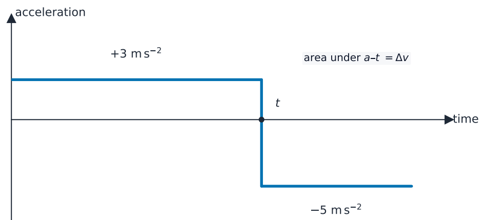
Acceleration–time graph derived from the same motion
