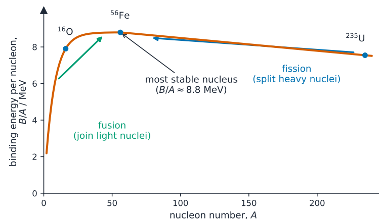
binding energy per nucleon peaks near ^{56}\text{Fe}
