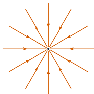
point mass
