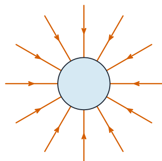
uniform sphere
