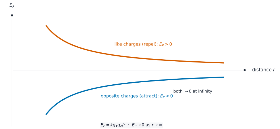
Electric PE of two charges: positive for like charges, a negative well for opposite charges
