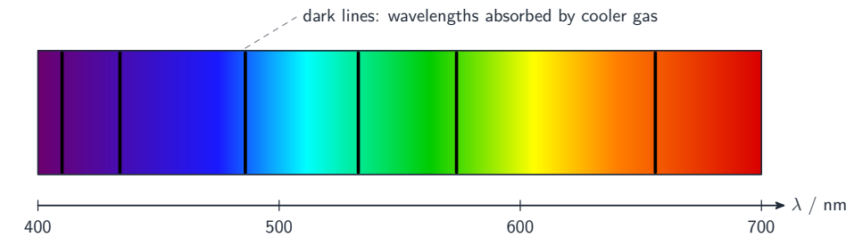
Dark absorption lines in the Sun’s spectrum mark the wavelengths absorbed by cooler gas
