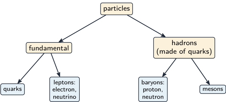
Fundamental particles (quarks, leptons) versus hadrons (baryons, mesons)
