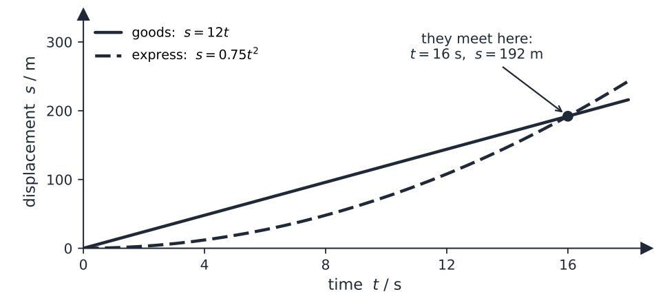
Meet where the displacement–time graphs cross (same s at same t )
