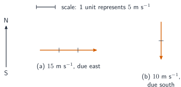
Vectors represented as arrows drawn to scale
