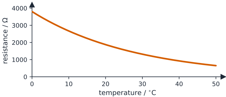
NTC: R falls as T rises
