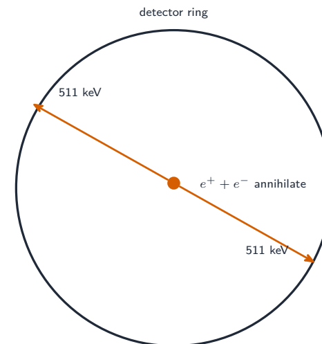
two photons, opposite directions — the coincidence fixes the line
