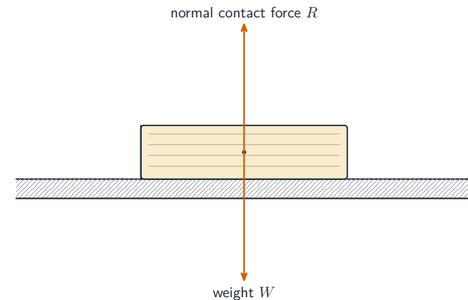
Weight and normal contact force on a book resting on a table
