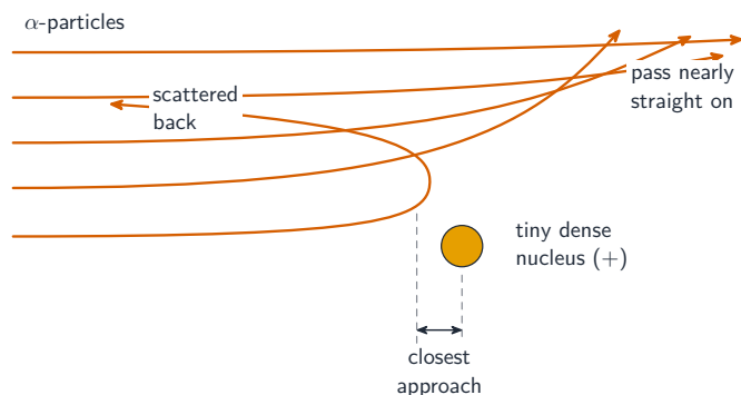
The \alpha -scattering experiment — \alpha -particles strike a thin gold foil in a vacuum
