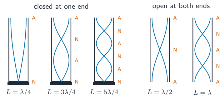
Modes of an air column: a closed end is a node, an open end an antinode
