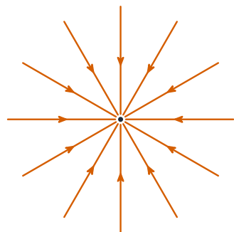
point mass
