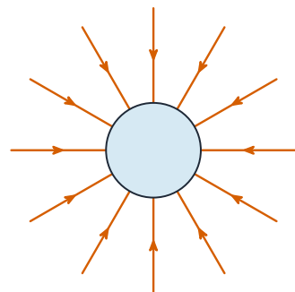
uniform sphere
