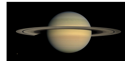
Saturn, its rings (countless small orbiting pieces) and its moons are all held in orbit by gravity
