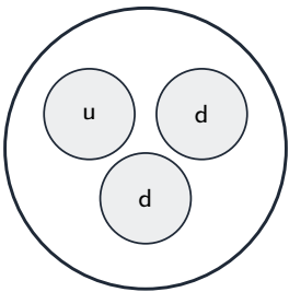
neutron (charge 0)
