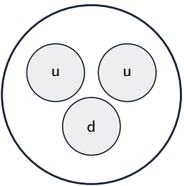
proton (charge +1)
