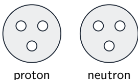
proton
