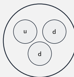
neutron (charge 0)
