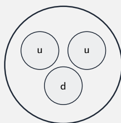
proton (charge +1)
