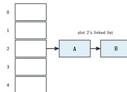
chaining
