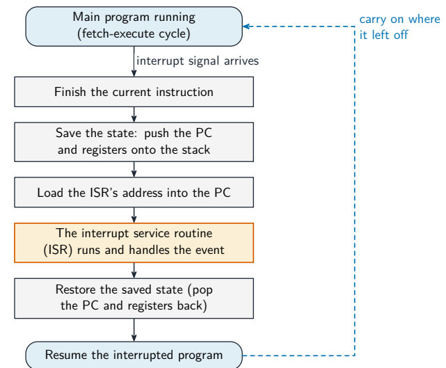
How an interrupt fits into the fetch-execute cycle
