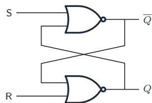
two NOR gates, each output fed back to the other's input
