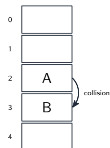
linear probing
