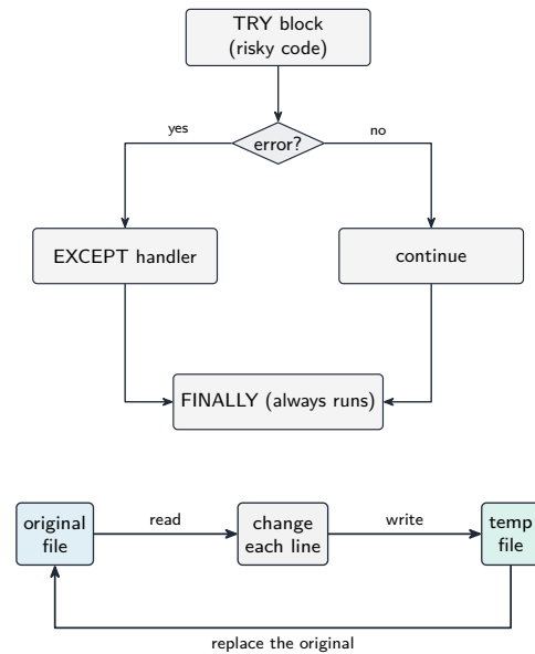
Updating a file record with exception handling
