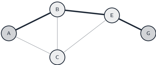
the shortest path A \rightarrow B \rightarrow E \rightarrow G is highlighted
