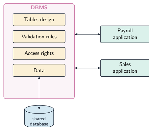
A DBMS replaces the older file-based approach to data
