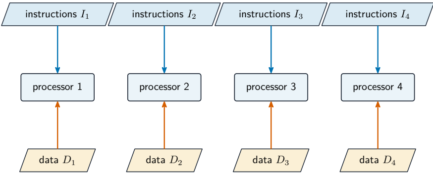
MIMD: each processor runs its own instructions on its own data
