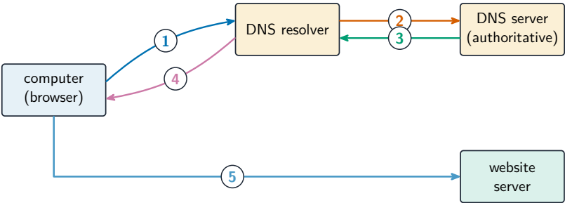
1 computer asks the resolver for the IP 2 resolver queries a DNS server 3 server returns the IP address 4 resolver passes the IP back to the computer 5 browser connects to that IP and requests the page
