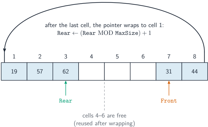
A circular queue wraps the pointers back to the start of the array
