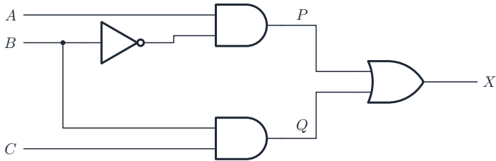
Label every intermediate output: here P is A AND NOT B and Q is B AND C, so X is P OR Q
