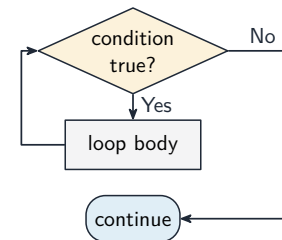
WHILE: test first
