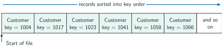
Sequential file: records are sorted by a key field
