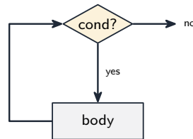
iteration
