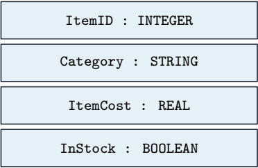
record TStockItem
