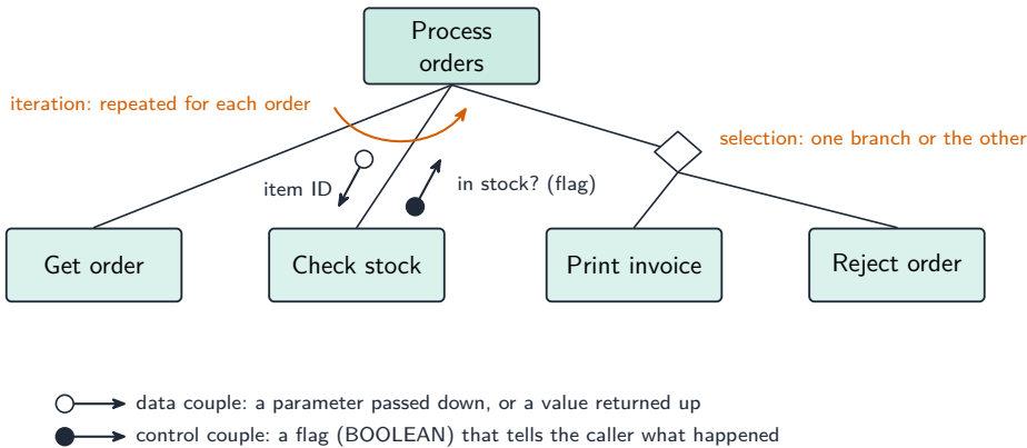
The structure-chart symbols: data and control couples, a selection diamond and an iteration arrow
