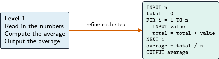
Stepwise refinement: expand each high-level step into detailed pseudocode
