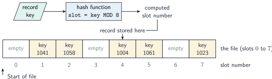
Random file: records sit at positions computed from the key
