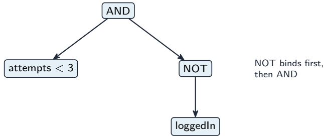
Precedence: NOT binds to loggedIn first, then AND combines the two sides
