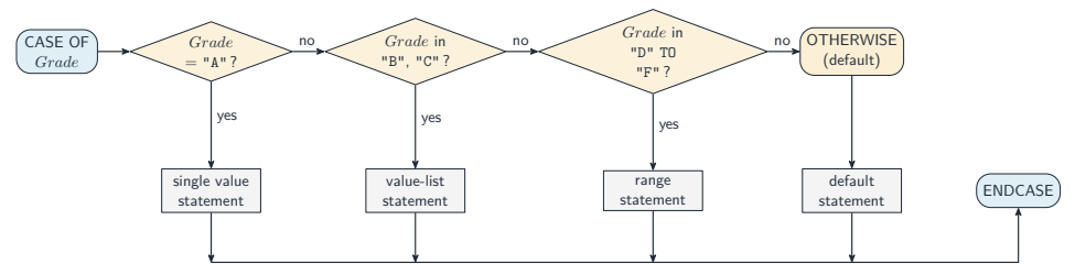
A CASE statement runs the branch that matches the value
