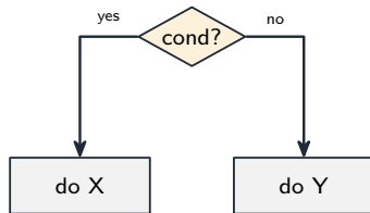
selection
