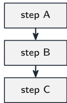
sequence
