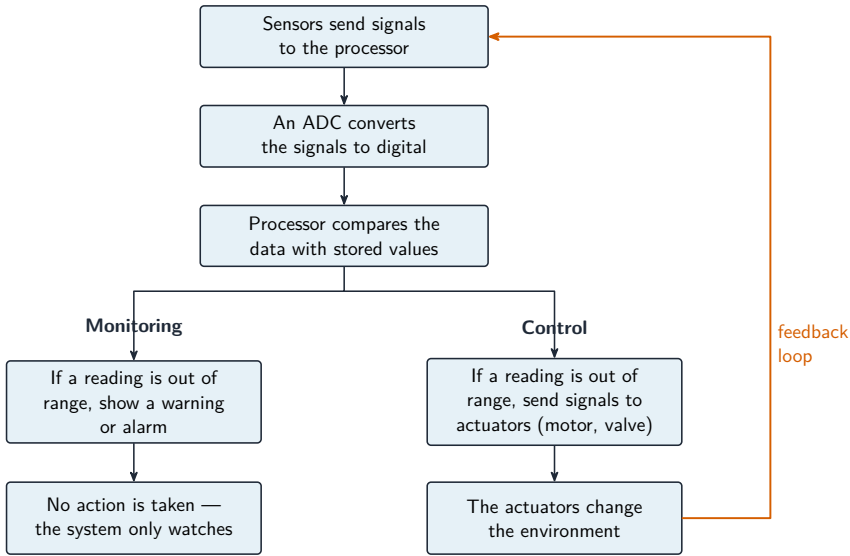
Monitoring reports data; a control system acts through a feedback loop
