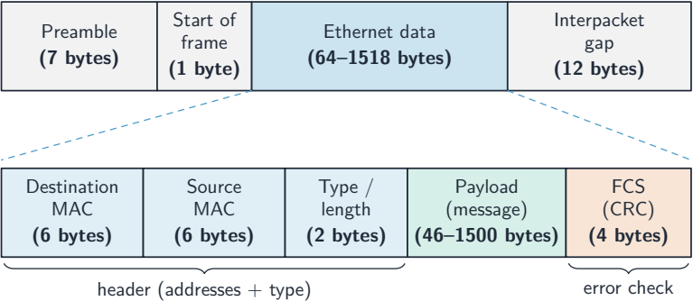
The parts of a typical Ethernet frame
