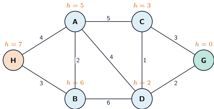
edge numbers: actual distances; h (red): the heuristic estimate of the distance still to go to G, used only by A*. Start at H (Home), goal G (School)
