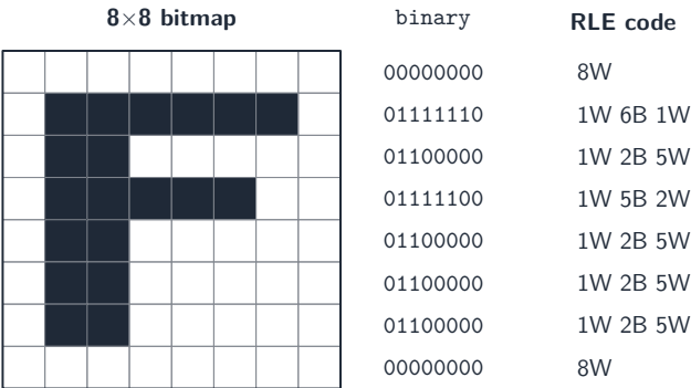
Key: 1 = black (B), 0 = white (W). RLE stores count + colour : e.g. 01111110 → 1W6B1W
