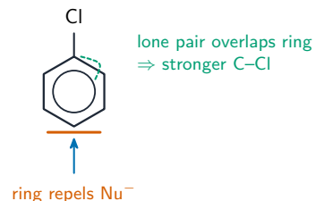
chlorobenzene: unreactive
