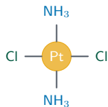
trans (opposite)
