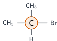
secondary 2 C
