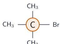
tertiary 3 C
