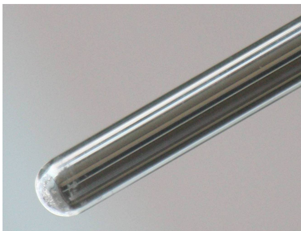
A positive Tollens' test: an aldehyde coats the tube with a shiny silver mirror
