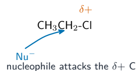
chloroethane: reactive
