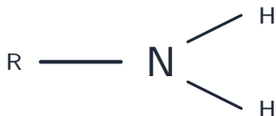
primary ( \text{-NH}_2 )
