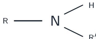
secondary ( \text{-NH-} )
