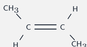
trans (opposite)
