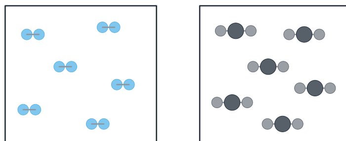
hydrogen, \text{H}_2
