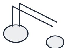
distillation (stops at aldehyde)
