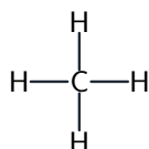
methane \text{CH}_4
