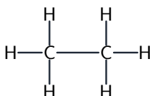
ethane \text{C}_2\text{H}_6
