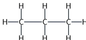
propane \text{C}_3\text{H}_8
