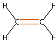
ethene \text{C}_2\text{H}_4 unsaturated: C=C double bond
