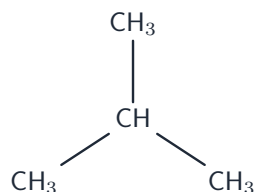
2-methylpropane (branched)
