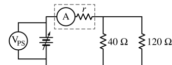
Circuit 3
