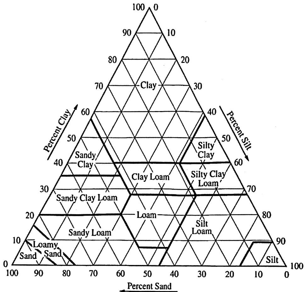
SOIL TEXTURE TRIANGLE
