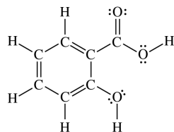
Salicylic Acid Melting Point: 159^{\circ}\text{C}
