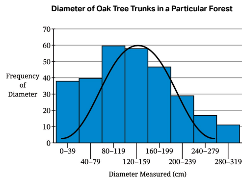
Figure 2. Histogram
