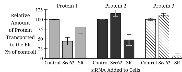
Figure 2. Average relative amounts of three proteins that were transported to the ER when treated with control siRNA, Sec62 siRNA, or SR siRNA. Error bars represent \pm SE_{\bar{x}} .
