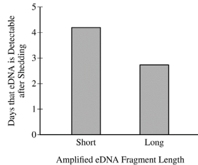
Figure 1. Detectability of eDNA fragments of varying lengths
