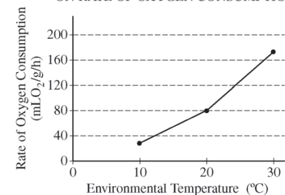
EFFECT OF ENVIRONMENTAL TEMPERATURE ON RATE OF OXYGEN CONSUMPTION
